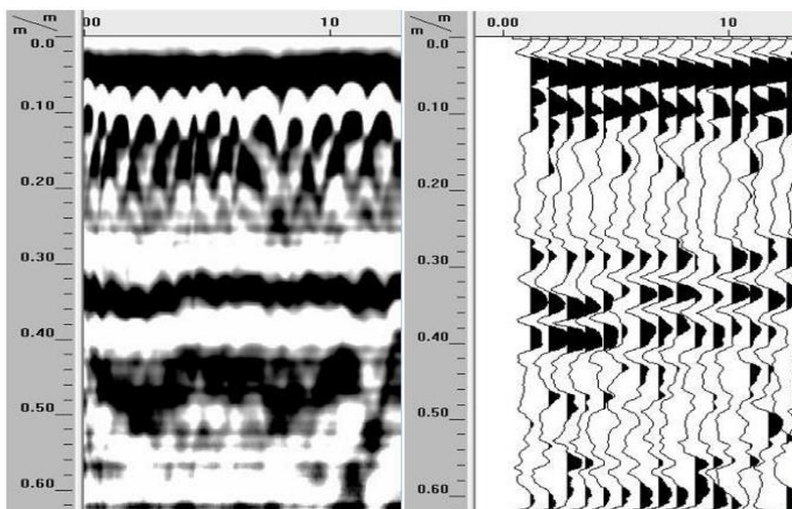
Figure 4. Characteristic map of void area of line 1.
